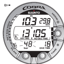
Fig. 3.12. Cylinder pressure warnings. Pressure has dropped below 50 bar [725 psi]. Pressure display is blinking and there is an audible alarm.
