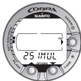
Fig. 4.16. Dive Simulation options. [2 SIMUL].
