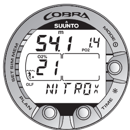
Fig. 3.21. Nitrox display. Maximum depth based on set O_2\% (21%) and PO_2 (1.4 bar) is 54.1 m [177 ft].
