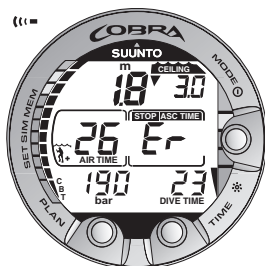
Fig. 3.19. Decompression dive, above ceiling. Note downward pointing arrow, Er warning and an audible alarm. You should immediately (within 3 minutes) descend to or below ceiling.
