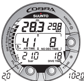
Fig. 3.9. Diving display. Present cylinder pressure is 210 bar [3045 psi] and remaining air time 41 minutes. Alternative display of current time and temperature is shown for 5 seconds after pressing TIME button.
