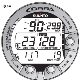
Fig. 3.13. Ascent Rate Indicator. Blinking depth reading, SLOW and four segments are shown together with an audible alarm: ascent rate is more than 10 m/min [33 ft/min]. This is a caution to slow down! STOP sign means that you are advised to make a Mandatory Safety Stop when you reach a depth of 6 m [20 ft].
