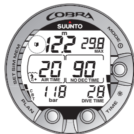
Fig. 3.10. Bookmark activation. An annotation, Bookmark, is placed in the profile memory during a dive by pressing PLAN button. Note Logbook symbol.
