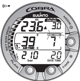
Fig. 3.16. Decompression dive, below floor. Upward pointing arrow, blinking ASC TIME label and an audible alarm tell you to ascend. Minimum total ascent time including safety stop is 7 minutes. Ceiling is at 3 m [10 ft].
