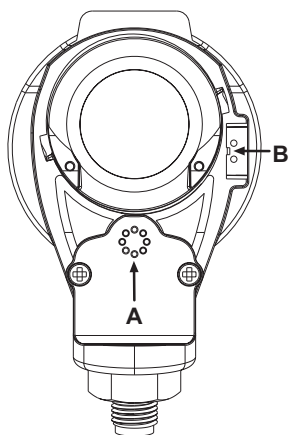
Fig 2.3. Depth sensor (A), water/data transfer contacts (B).
