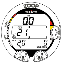
Fig. 3.21. Surface display in the Nitrox mode
